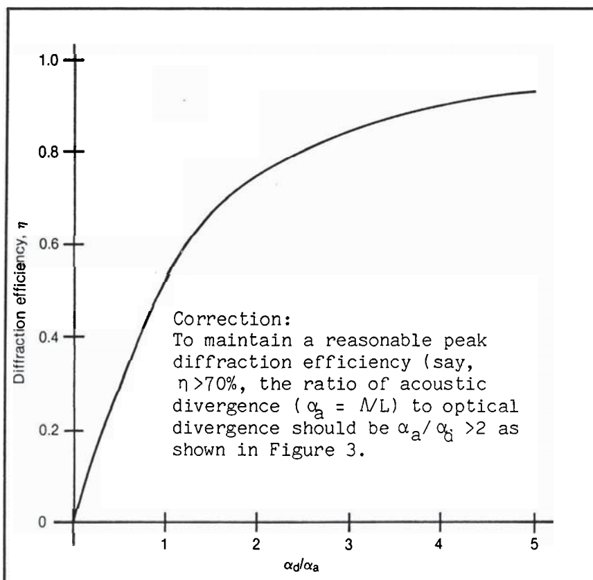
Figure 3. Diffraction efficiency as a function of optical and acoustic divergence.
