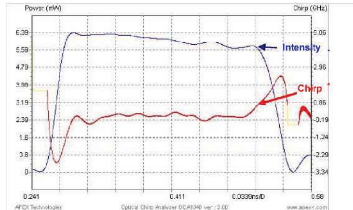
Figure 8: Intensity and chirp measurement of a z-cut LiNbO3 external modulator measured by the Optical Complex Spectrum Analyzer
