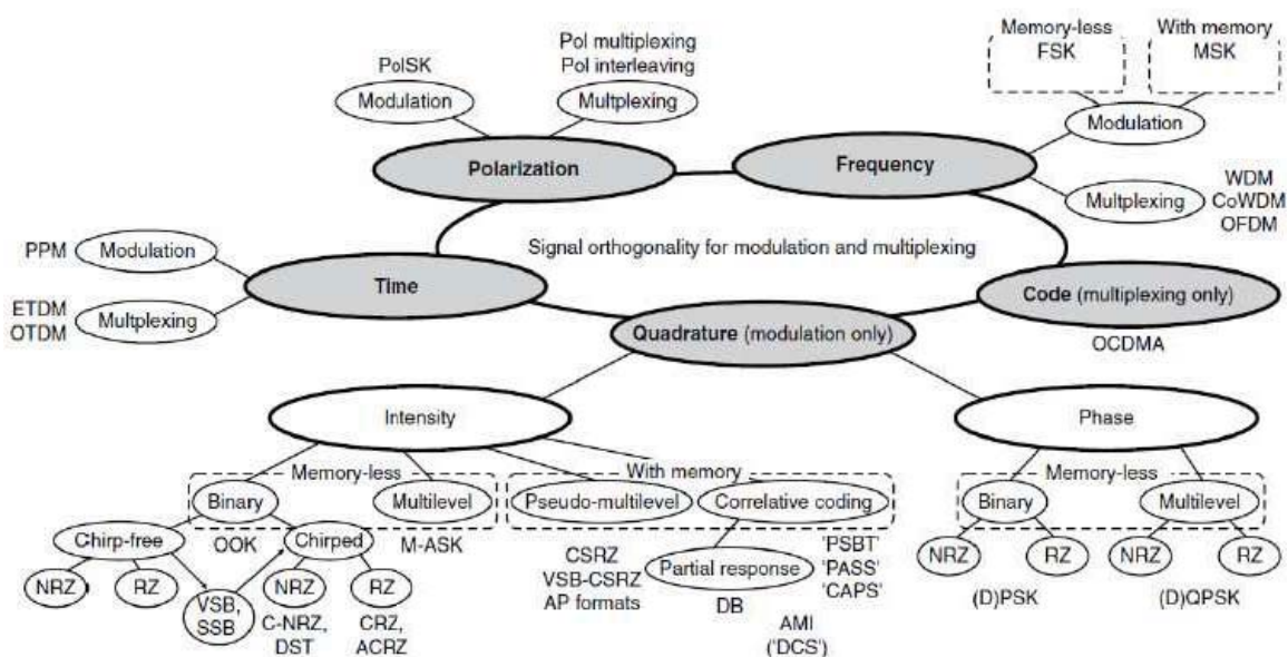
Figure 1: Classification of the most important modulation formats and multiplexing schemes used in optical communications systems
