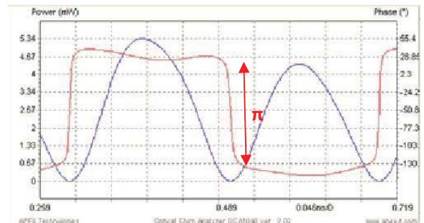
Figure 6: 10 Gb/s Duobinary modulation Intensity (blue trace) and phase (red trace) measured by the Optical Complex Spectrum Analyzer
