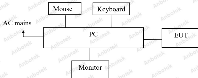
For Mode 1 Block Diagram of Test Setup
