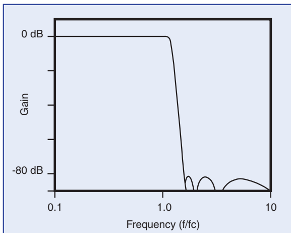
SR640 gain response
