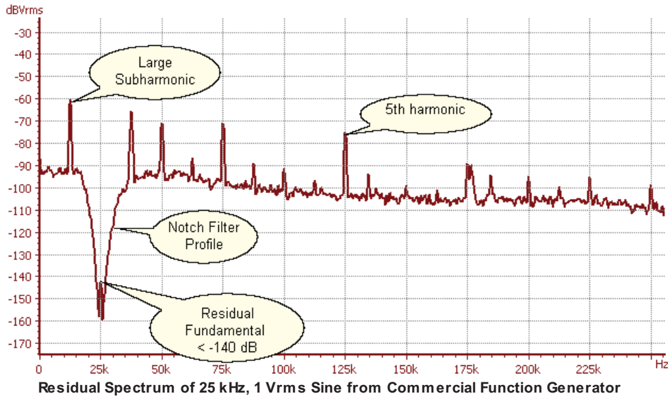
Residual Spectrum of 25 kHz, 1 Vrms Sine from Commercial Function Generator
