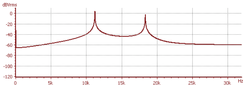
Unwindowed Spectrum
