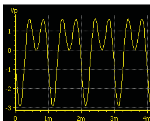
...And Inverted
