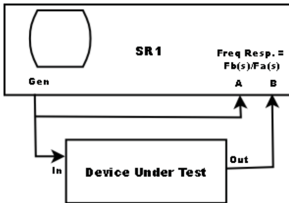
Typical Dual-Channel Response Measurement
