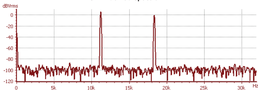
Spectrum with BlackmanHarris+ Window
