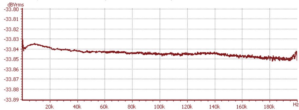
Chirp, Hi-Bandwidth ADC (Y-scale = 10 mDb/div)
