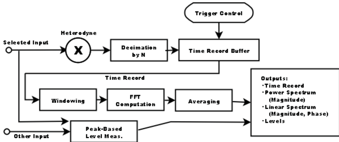
FFT1 Analyzer Block Diagram
