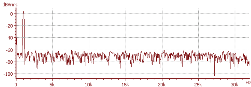
Unaveraged Power Spectrum of Sine+Noise
