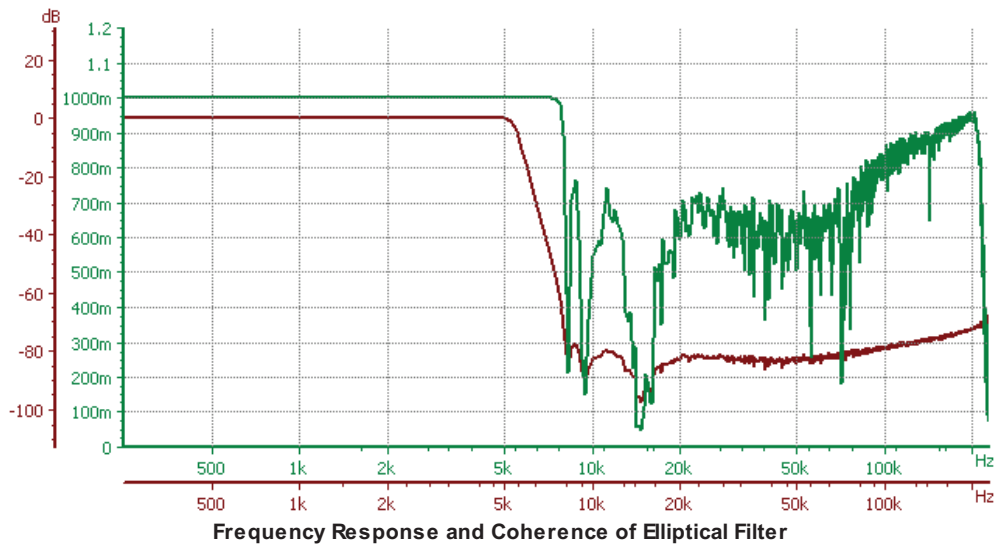
Frequency Response and Coherence of Elliptical Filter
