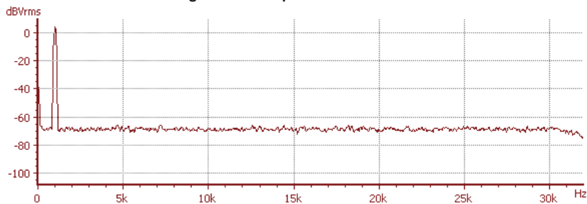
Averaged (N=10) Power Spectrum of Sine+Noise
