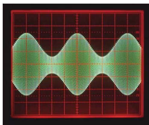
Amplitude modulation
