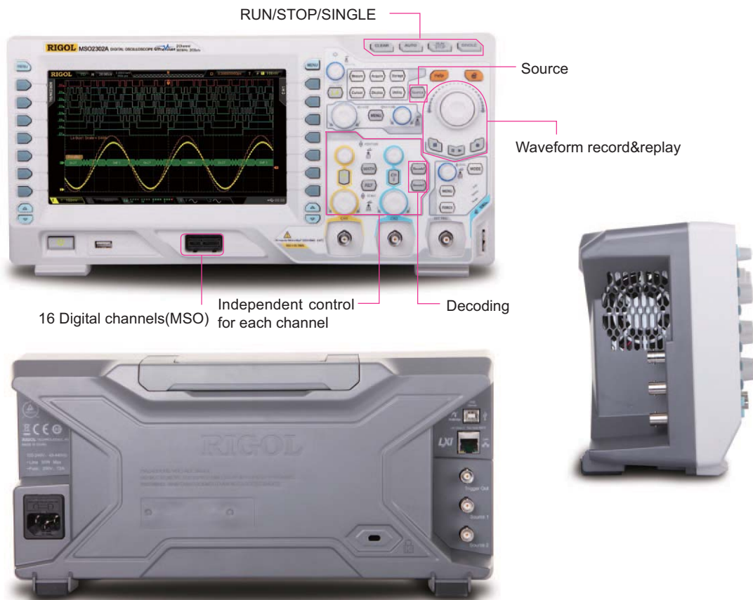
Product Dimensions: Width X Height X Depth=361.6 mm×179.6 mm×130.8 mm Weight: 3.9 kg ± 0.5 kg(Without Package)
