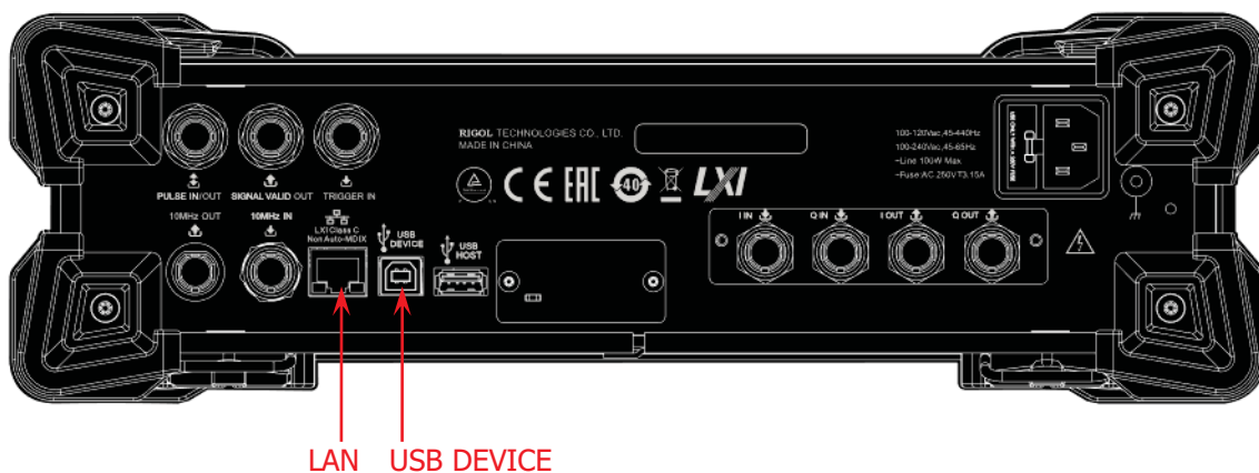
Figure 1-1 DSG3000B Communication Interfaces
