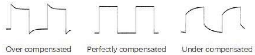
Figure 5.7 Probe Compensation
