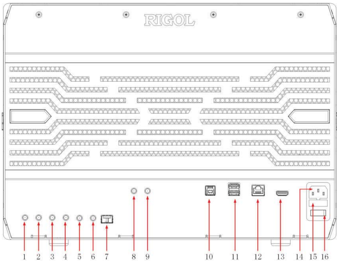
Figure 4.2 Rear Panel
