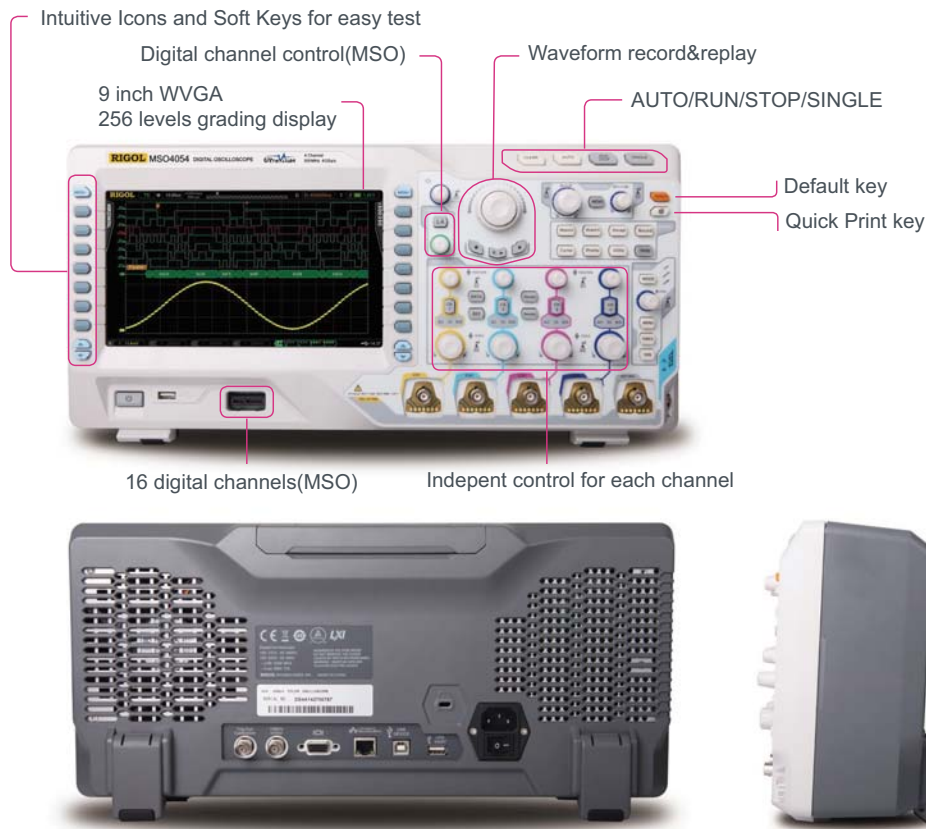
Product Dimensions: Width X Height X Depth = 440.0mm X 218.0 mm X 130.0 mm Weight: 4.8 kg ± 0.2 kg (Without Package)
