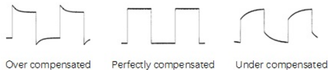
Figure 5.6 Probe Compensation
