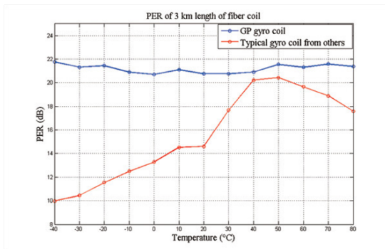
Fig. 3: PER vs. temperature of a 3 km coil from GP (blue) and another vendor (Red). PER variation over a 120°C temperature range: <2dB (GP) vs. >10 dB (others)
