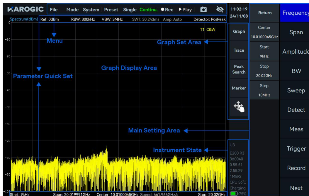
Figure 1 SASTudio4 UI layout
