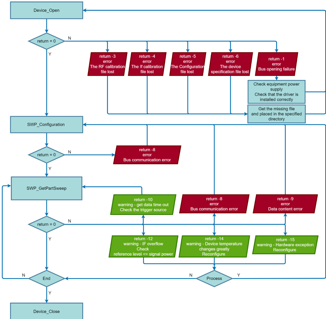
Figure 54 SWP mode call flow chart.
