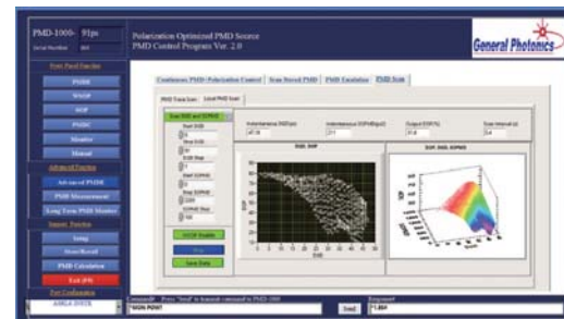
Figure 4. 3D graph display of a DGD/SOPMD scan
