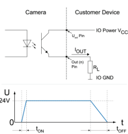
Digital Output: High Active
